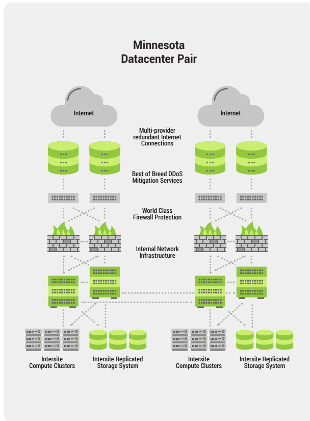
Infinite Campus Data Centers
