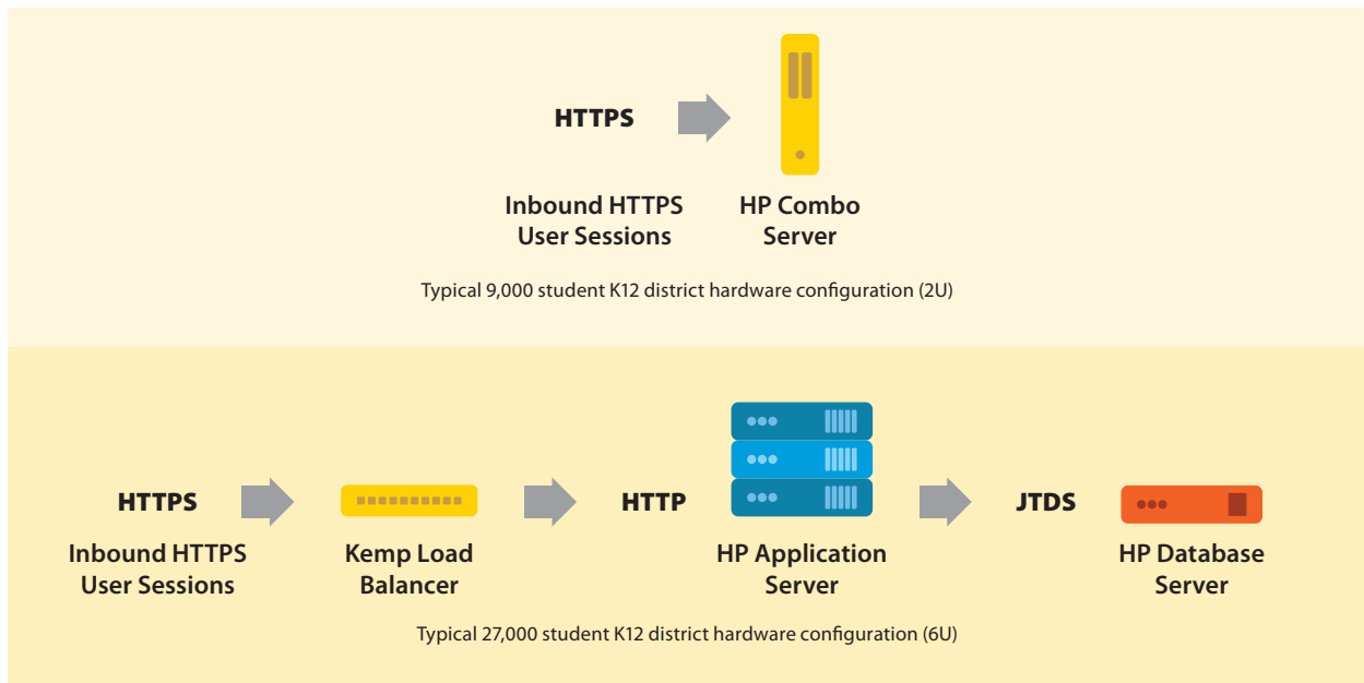
Typical Onsite Hosting configuration
